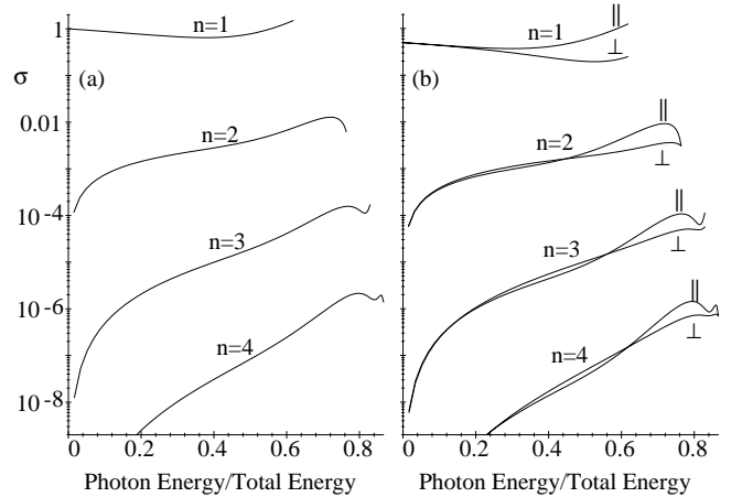
FIG. 5. Calculated spectra, \sigma \equiv (\omega \mathcal{E} / \pi r_0^2 m^2) (dW_n / d\omega') , of backscattered photons produced in the interaction of a 46.6 GeV electron with n = 1, 2, 3, and 4 photons from a linearly polarized 527 nm plane wave with \eta = 0.1 , as a function of the ratio \omega' / \mathcal{E} of the energy of the backscattered photon to that of the beam electron. (a) Spectra summed over the polarization of the backscattered photon. (b) Spectra for polarization of the backscattered photon parallel and perpendicular to that of the incident wave.
