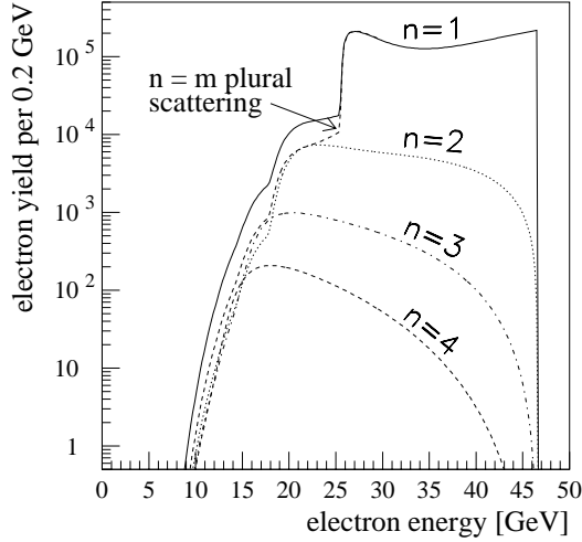
FIG. 4. The calculated rate of scattered electrons for linear, nonlinear and plural Compton scattering for the infrared laser and electron beam parameters given in the text. The solid line is the sum of all possible processes. The rates for n = 2, 3, and 4 nonlinear Compton scattering are shown separately as well.
